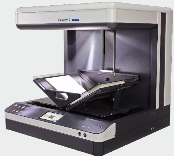
Book cradle in 120° V position.
